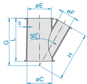
■ Conical lateral 30°
