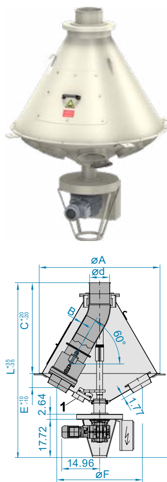
1 Drain nozzle
