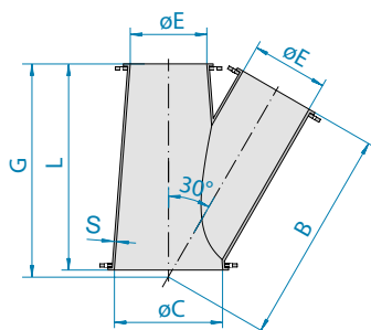
Conical lateral 30°
