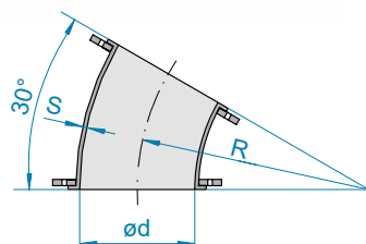
1 pressed bend 30°
