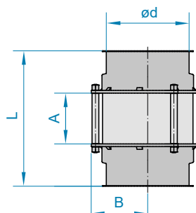
ND 3" to 6"
