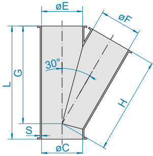
Lateral 30°
