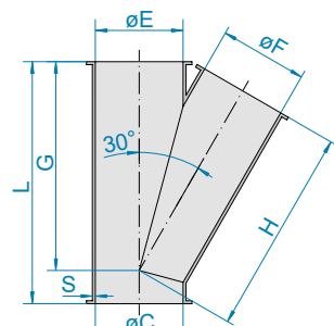
Lateral 30°
