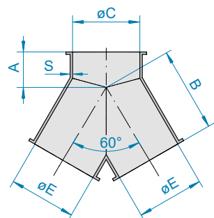
Y-branch 60°
