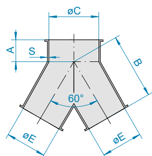
Conical Y-branch 60°
