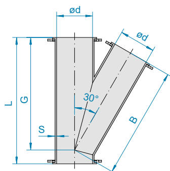
Lateral 30°
