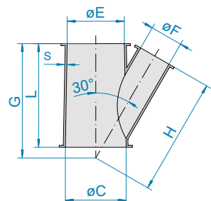
Conical lateral 30°
