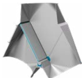
Cross-section: Two-way distributor 60° up to ND 12", symmetrical
