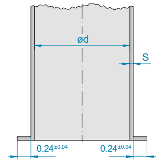
JACOB tubing system with a lip for pull ring connection
